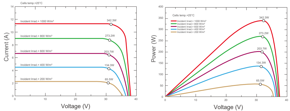
Current-Voltage &amp; Power-Voltage Curves (RMHT54/34001)
